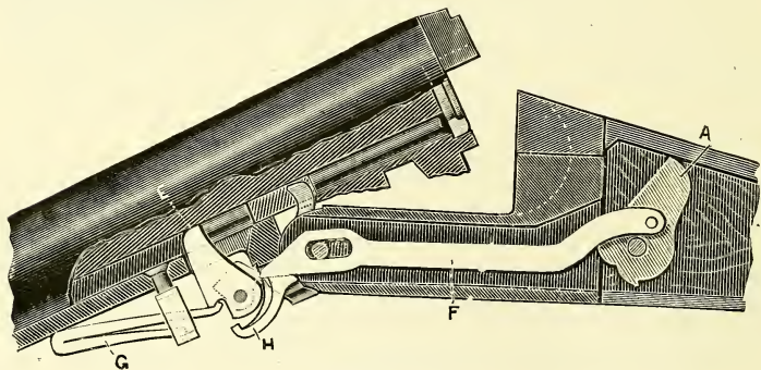
Ross's Ejector Gun.
